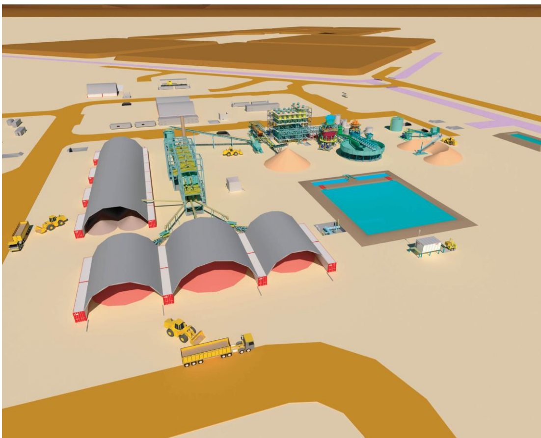
Figure 2 – PGGP Minerals sands modular plant and site layout (IHC Mining)
